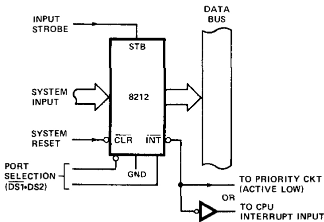
Figure 6. Interrupting Input Port
