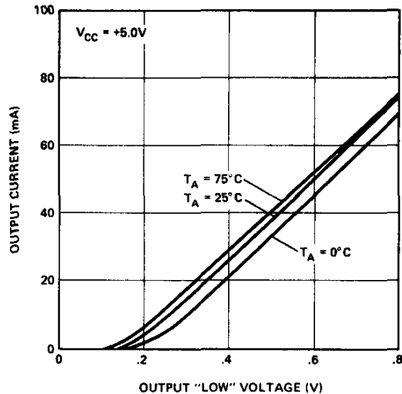
OUTPUT CURRENT VS. OUTPUT "LOW" VOLTAGE
