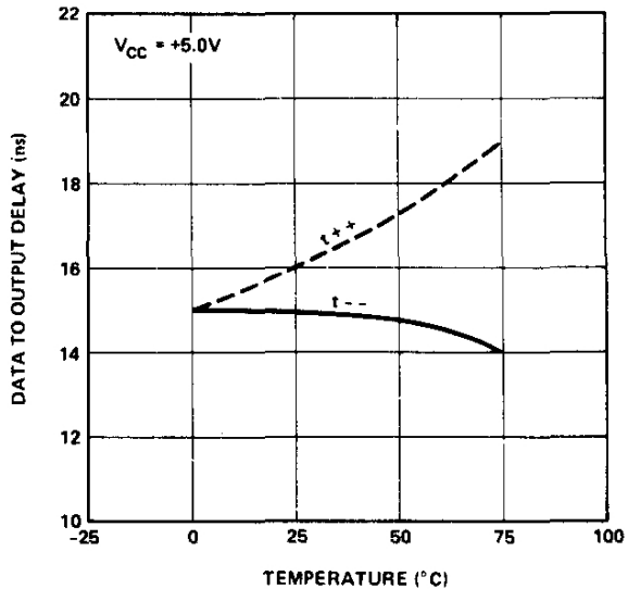
DATA TO OUTPUT DELAY VS. TEMPERATURE
