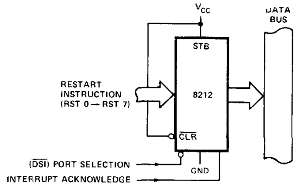
Figure 7. Interrupt Instruction Port
