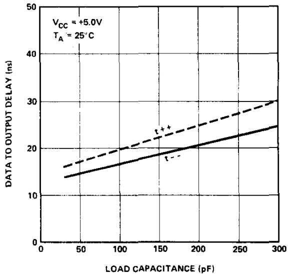
DATA TO OUTPUT DELAY VS. LOAD CAPACITANCE
