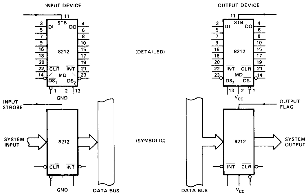
Figure 3. Basic Schematic Symbols
