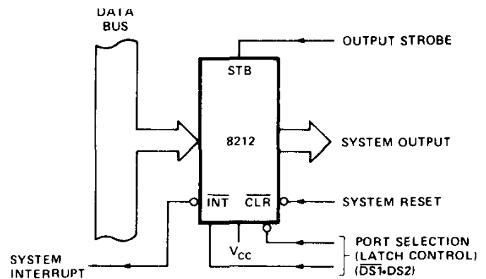
Figure 8. Output Port
