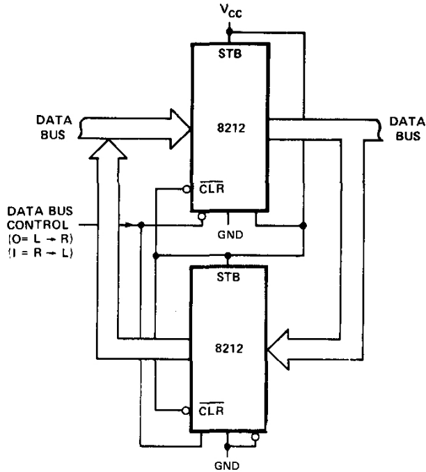
Figure 5. Bidirectional Bus Driver
