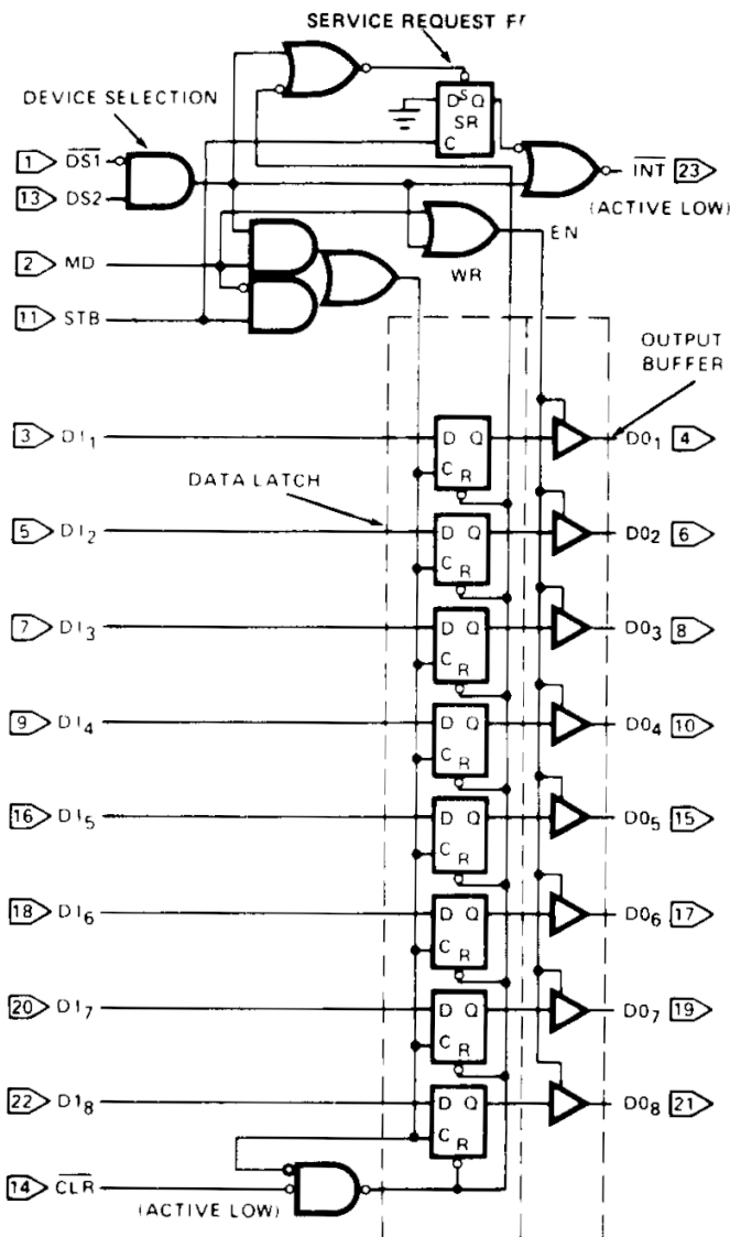
Figure 1. Logic Diagram
