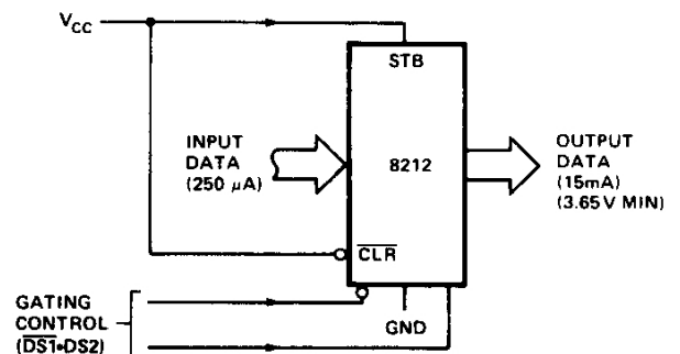
Figure 4. Gated Buffer
