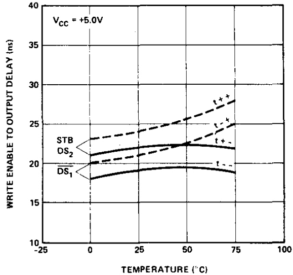
WRITE ENABLE TO OUTPUT DELAY VS. TEMPERATURE
