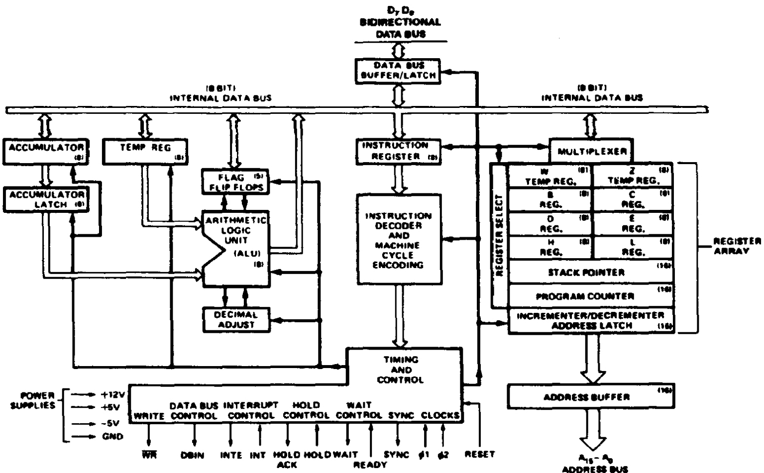
Figure 1. Block Diagram
