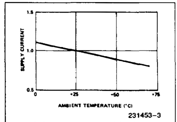
Typical Supply Current vs Temperature, Normalized \Delta I_{Supply} / \Delta T_A = -0.45\% / ^\circ\text{C}
