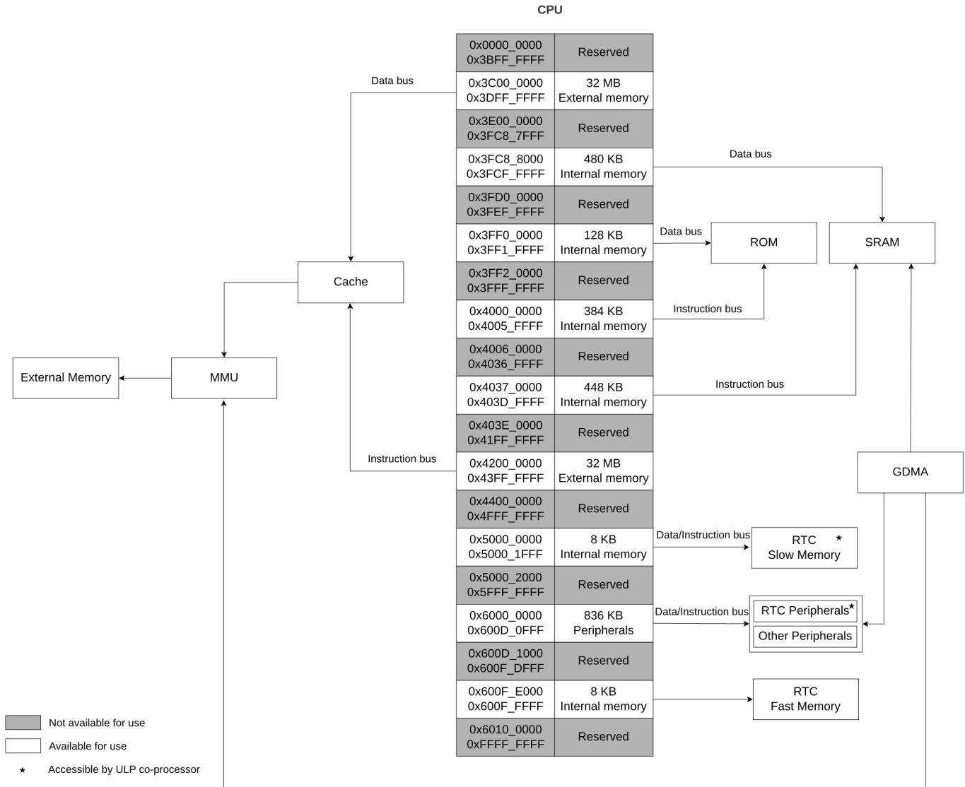
Figure 4-1. Address Mapping Structure
