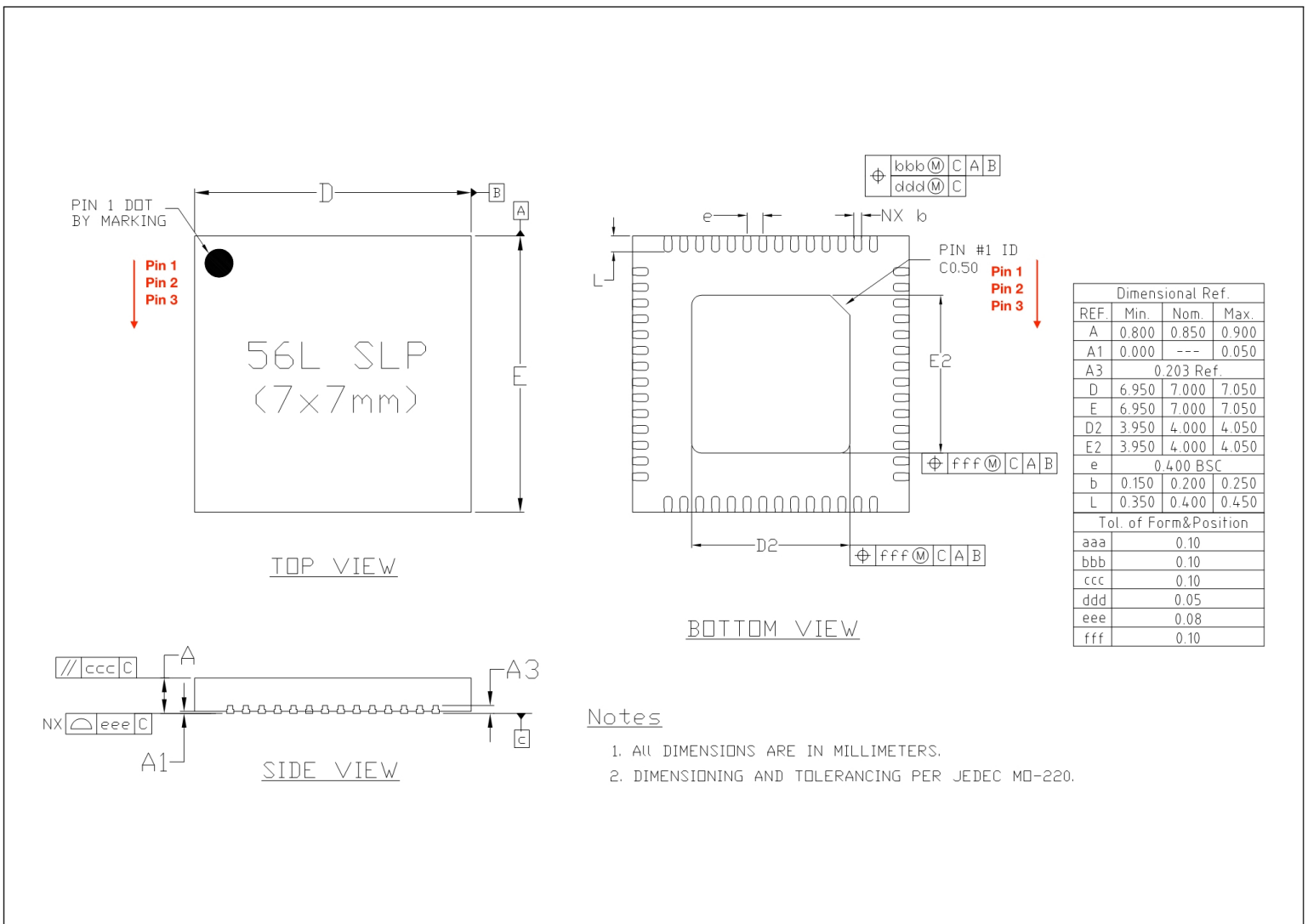
Figure 7-1. QFN56 (7x7 mm) Package
