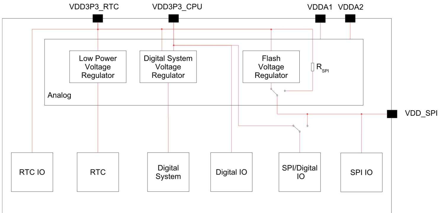
Figure 2-2. ESP32-S3 Power Scheme
