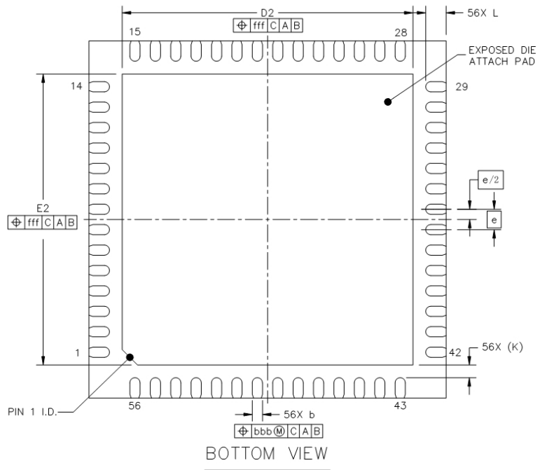
Figure 7-2. QFN56 (7×7 mm) Package (Only for ESP32-S3FH4R2)
