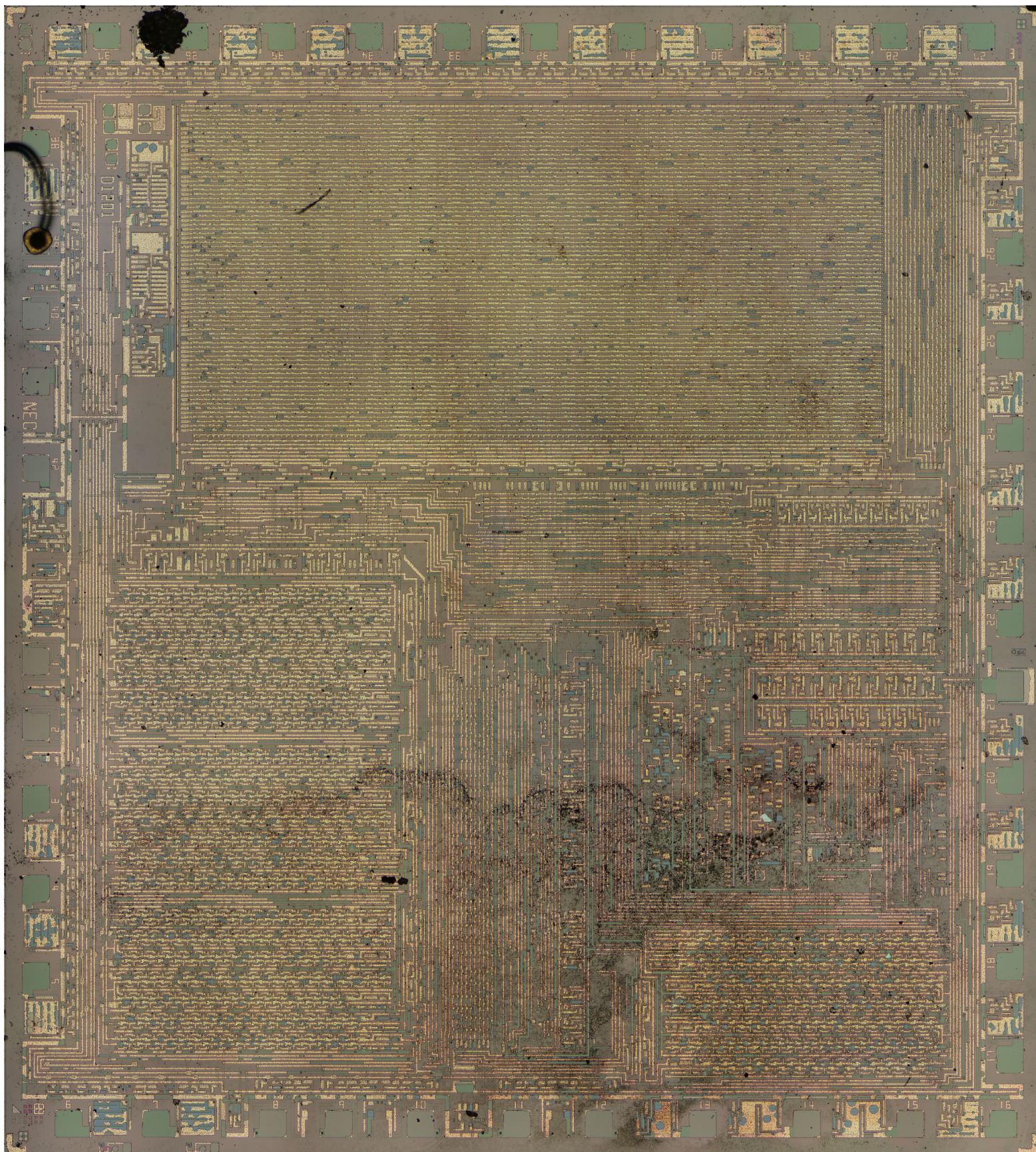
μPD1201C 20x Die Photo 14000 x 15528 (217 MP) 6400% (64x) Tolerant Synthesized by Hugin
