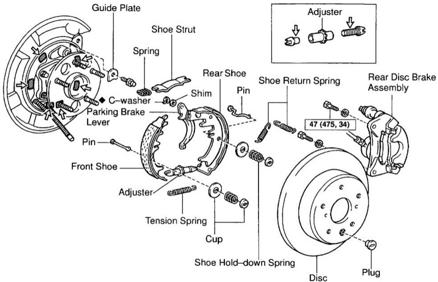
Parking brake & Disc brake combined mechanism
