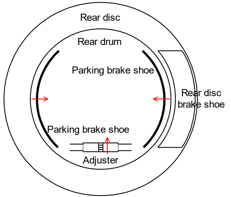
Loosen Parking Brake (Turn adjuster sprocket up)
