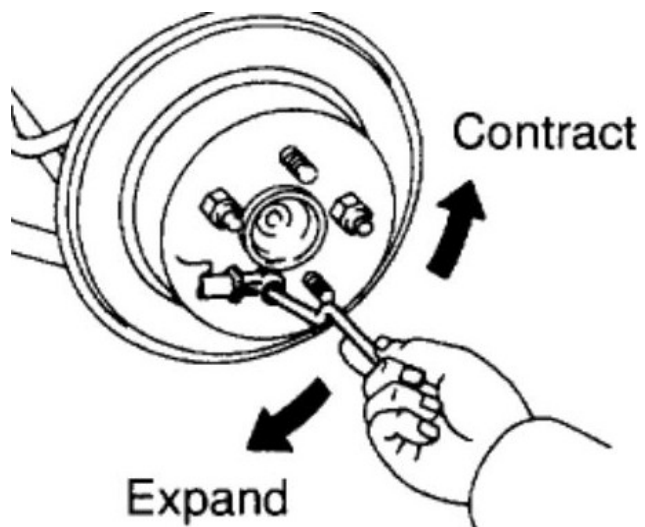
Rotate adjuster teeth up to loosen, down to tighten
