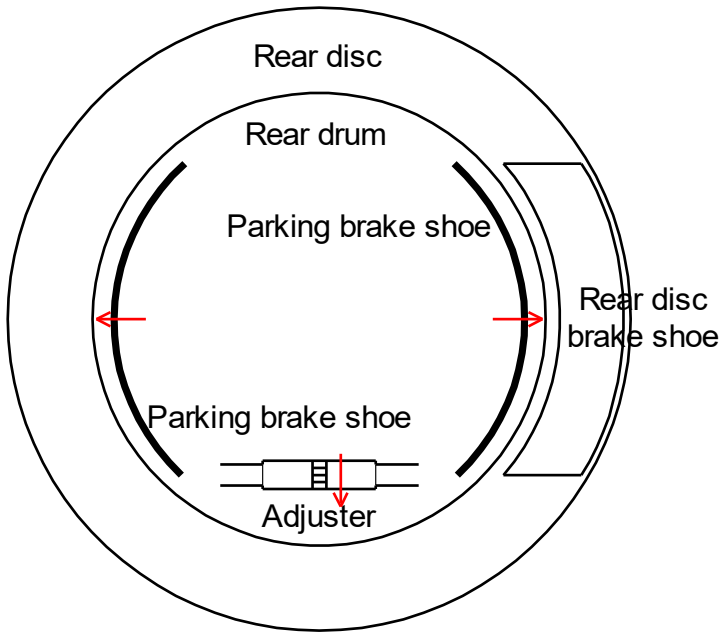
Tighten Parking Brake (Turn adjuster sprocket down)
