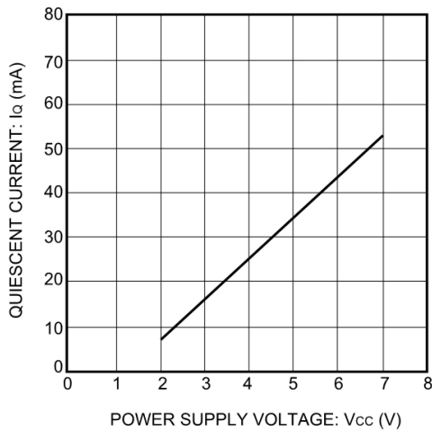
Fig. 10 Quiescent current vs. power supply voltage
