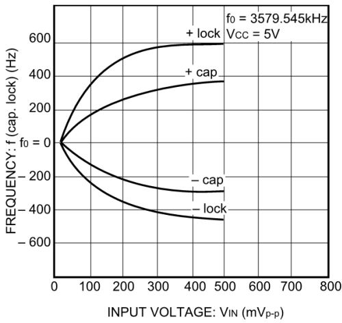
Fig. 13 Capture range and lock range ( \Pi ) vs. input voltage
