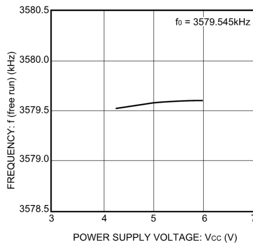
Fig. 11 VCXO free-run frequency vs. power supply voltage
