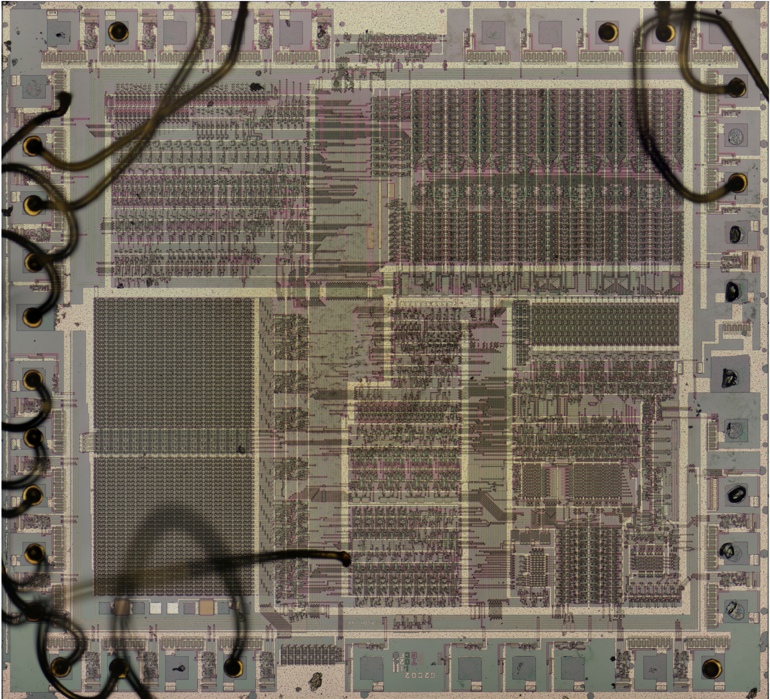
RP2C02 20x Die Photo 16458 x 15000 (247 MP) 6400% (64x) Tolerant Synthesized by Hugin
