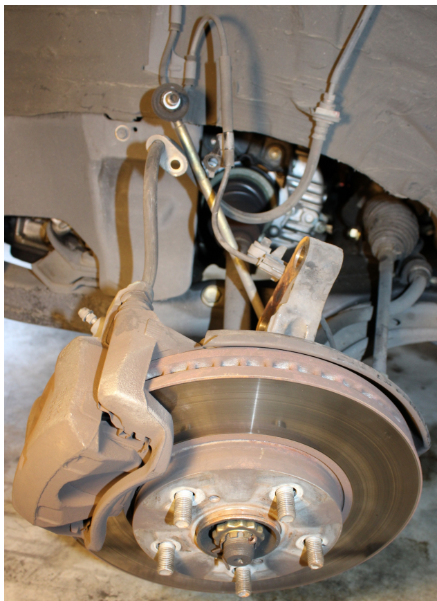
Removed (Passenger's side)
