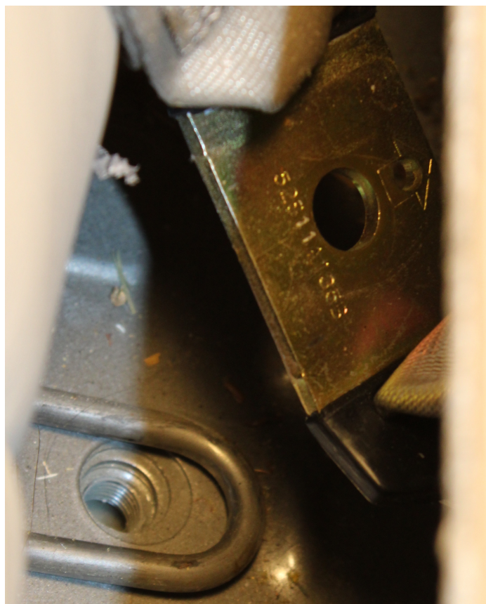
Remove bolt and sturdy washer connecting belt (two locations)
