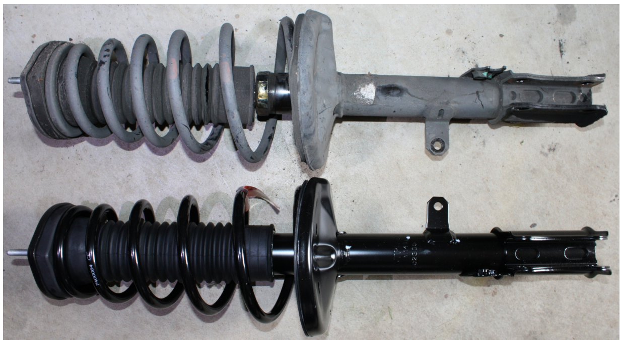
Passenger's side old (upper) & Driver's side new (lower) strut assembly (tab position differs)
