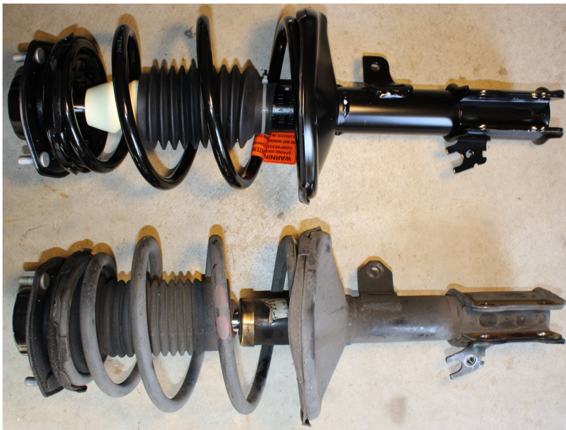
New (upper) and Old (Lower) strut assembly (Passenger's side)
