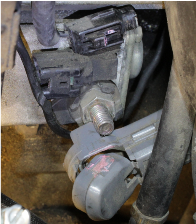
Power & control wire disconnected
