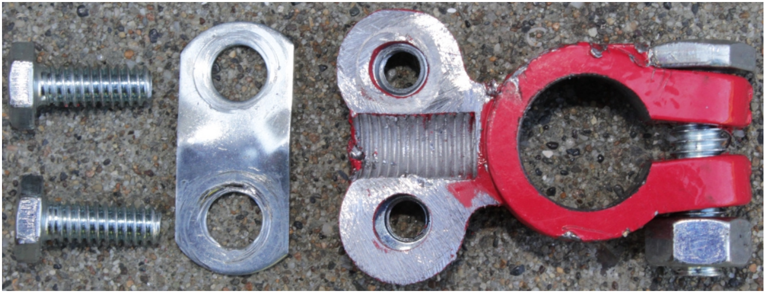
Filed to get sufficient electrical contact removing unnecessary red paint which is not conductive
