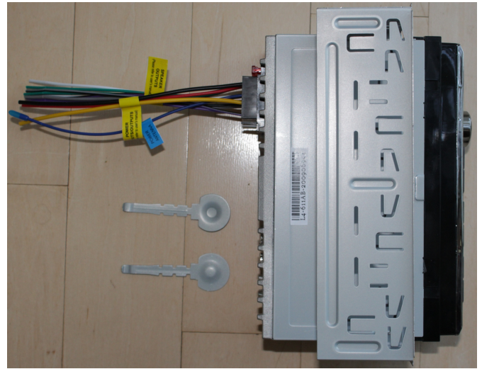
Radio, Mounting collar for attaching radio firmly to dash board opening (DIN), Bracket keys, Plastic trim
