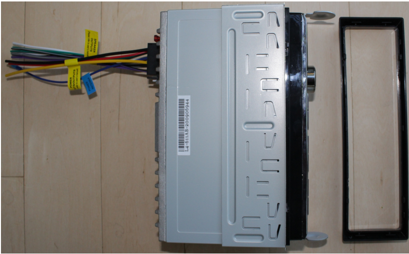
Radio, Mounting collar for attaching radio firmly to dash board opening (DIN), Bracket keys, Plastic trim
