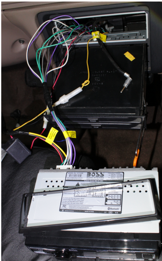
Wire connection completed by soldering Restoring radio & accessory into DIN (Deutsches Institut für Normung)
